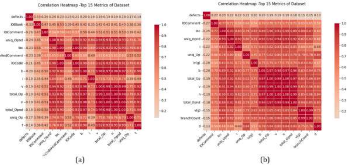
Fig. 9: Correlation Analysis on PC1 and CM1 Dataset with Gradient Boosting Classifier
