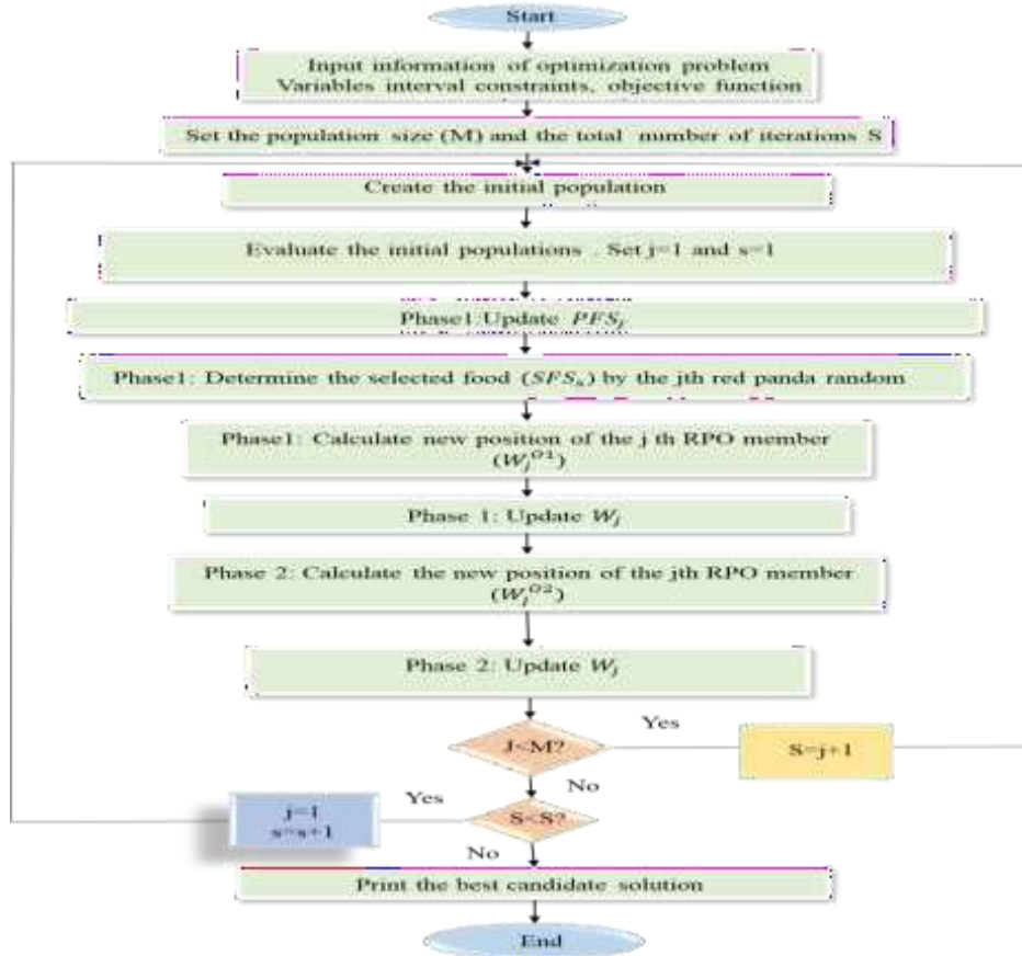
Figure 3: Flowchart illustrating the RPO algorithm process.
