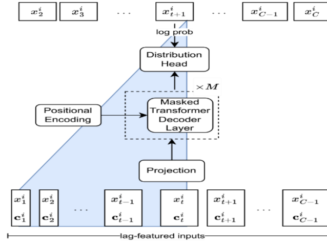
Figure 2: Lag-Llama architecture
