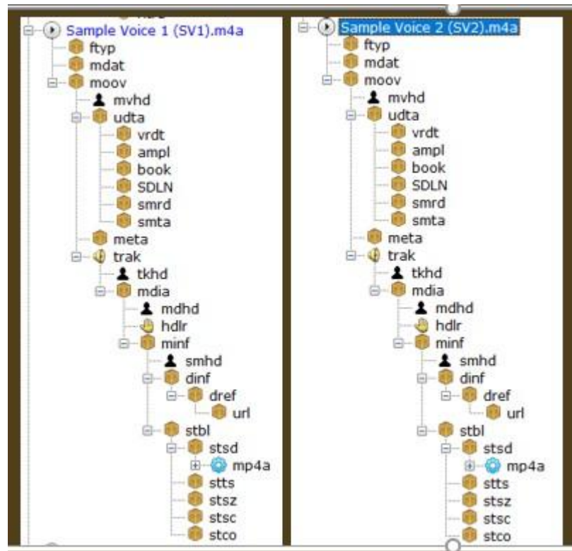
Figure5: Digital audio file container atoms and children atoms analysis of original audio recording recorded using inbuilt voice recorder of mobile phone-Samsung Note8 (left) and original recording shared via WhatsApp application of same phone.
