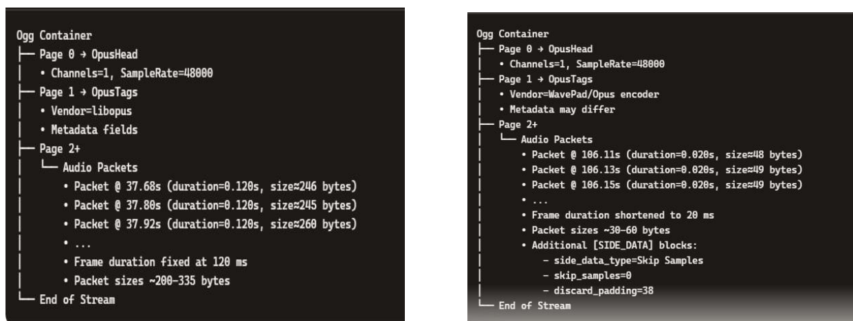
Figure 8: The parsed data of original digital audio files (left) vs tampered digital audio file (right) seen upon container structure analysis.
