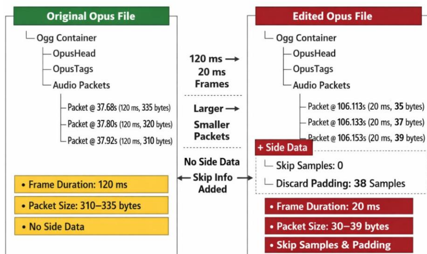
Figure 9: The left side window is container structure analysis of Original unaltered digital audio file and right side window shows the container structure analysis of tampered file.
