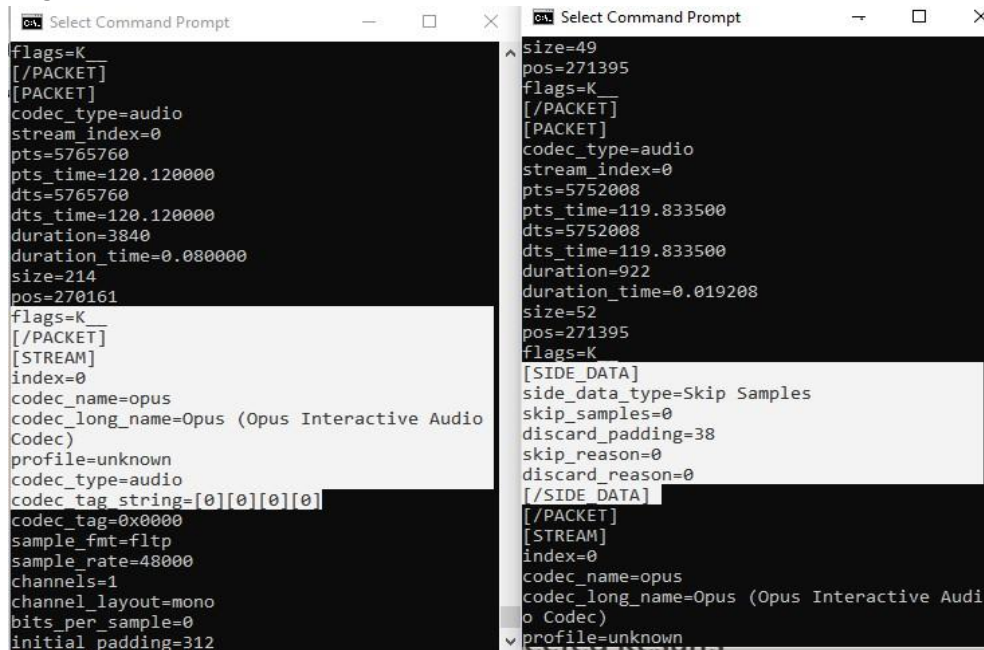
Figure 10: The left side window is a section of parsed data from Original file analysis and right side window shows the comparative section of parsed data from tampered file analysis.
