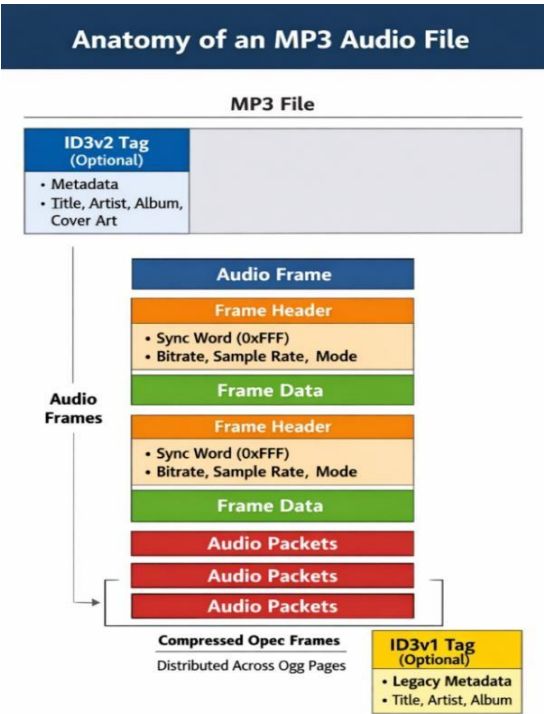
Figure 7: The core structure of a MP3 file.
