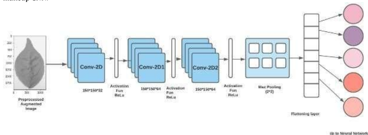
Figure. 2 CNN model architecture for leaf classification
