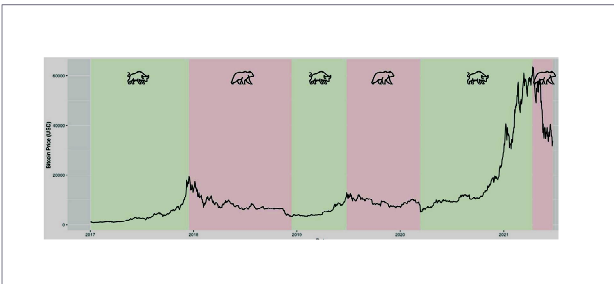
Figure 1: Bitcoin’s Price Evolution and Bull and Bear Market Identification
