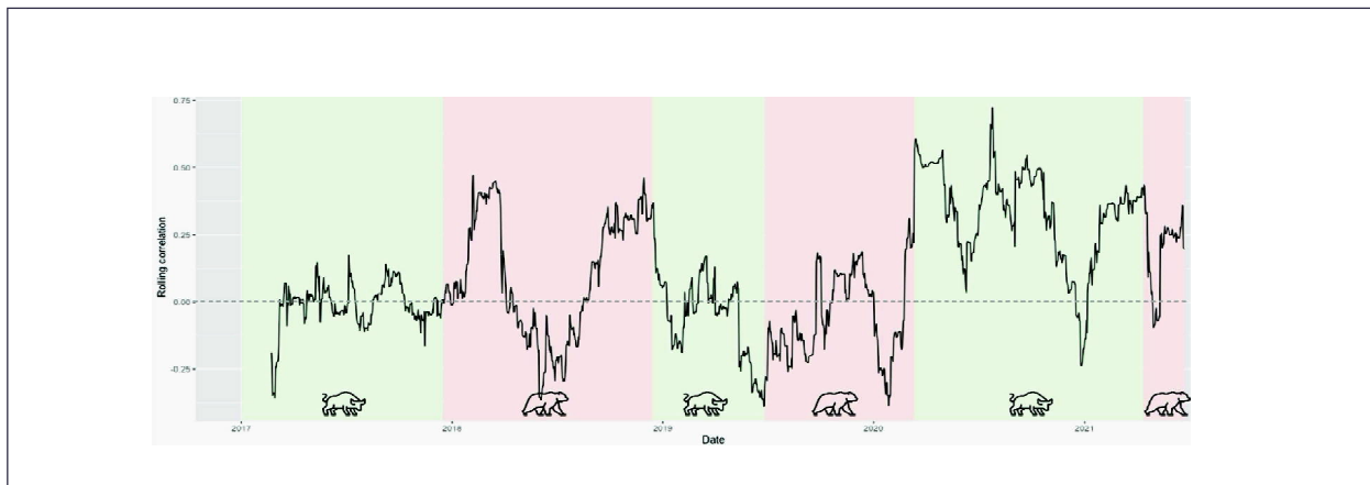
Figure 9: Rolling 50 Days Correlation for BTC and Dow Jones Index ETF
