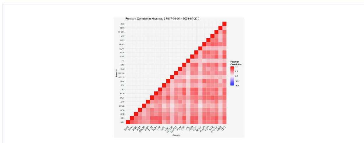
Figure 2: Correlation Heatmap for the Full Period
