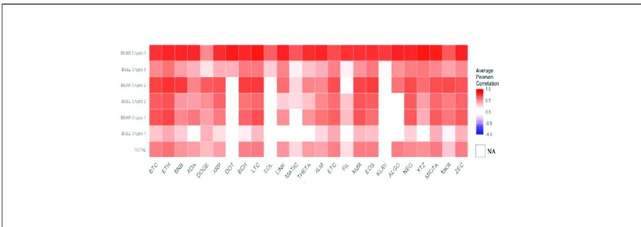
Figure 4: Average Correlation for Bull and Bear Periods
