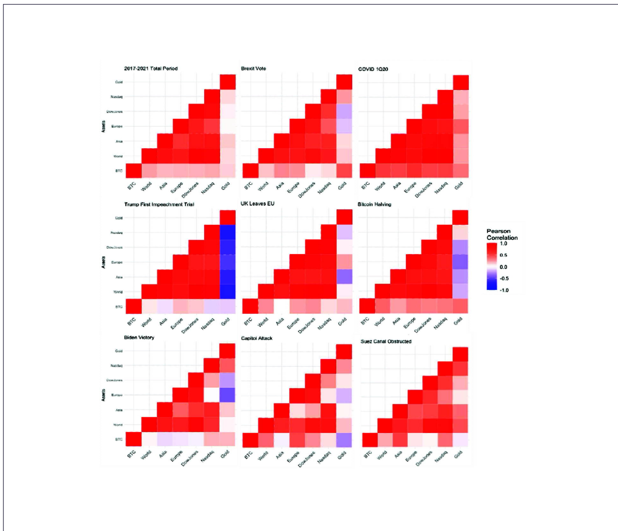
Figure 5: Pearson Correlation Heatmap for Relevant Macro Periods
