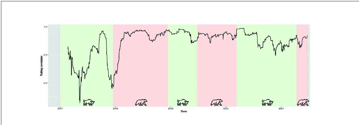
Figure 6: Rolling 50 Days Correlation for BTC and ETH
