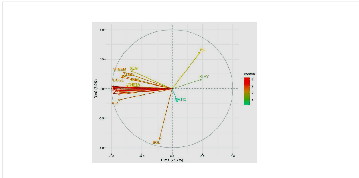
Figure 13: PCA: Variables' Contribution to Principal Components 1 and 2
