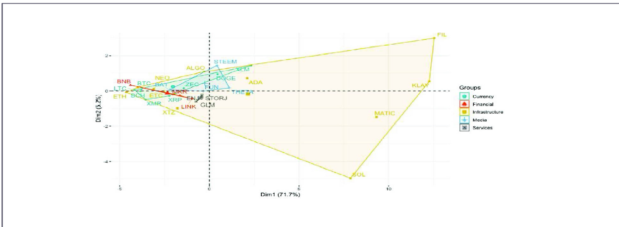
Figure 17: PCA: Elements Association based on Categories (PC1 and PC2)
