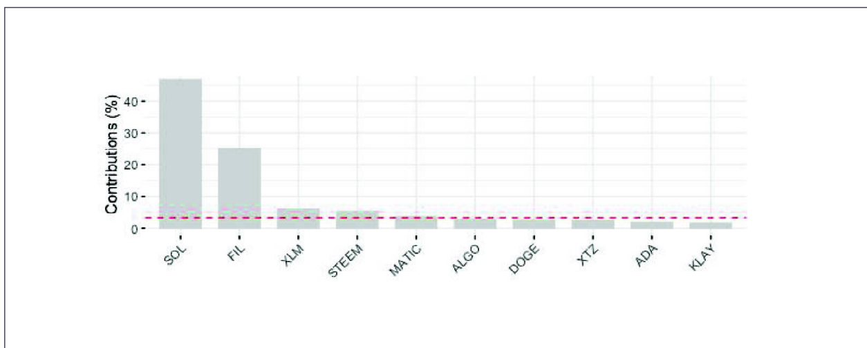
Figure 15: Contribution of Each Variable to Dimension 1 (Percentage terms)
