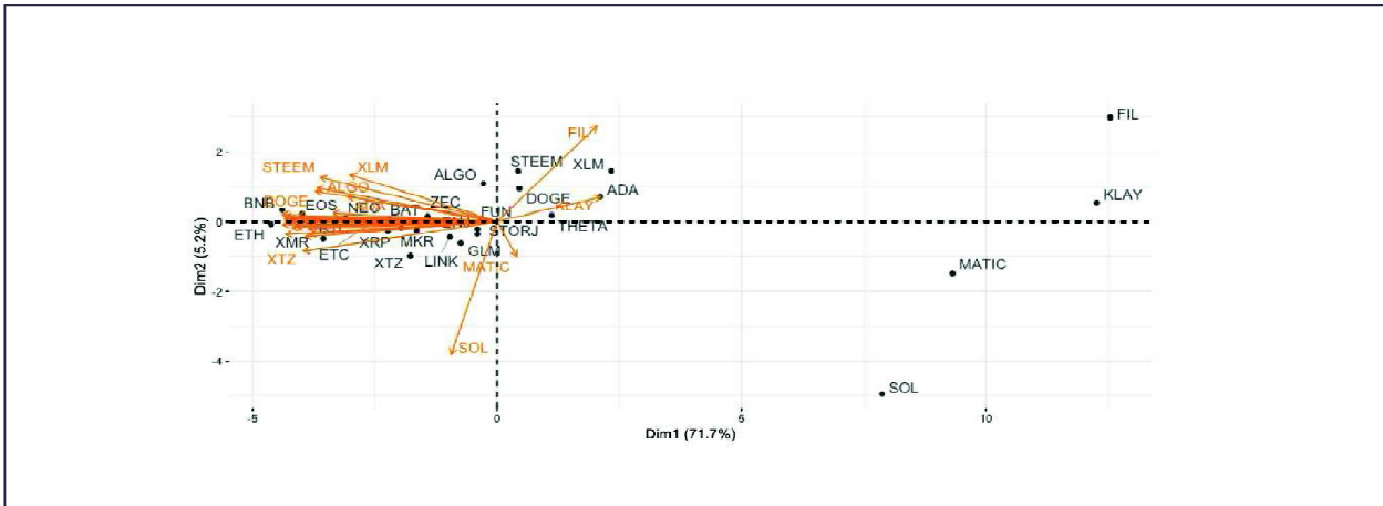
Figure 16: PCA: Variables and Elements as of PC1 and PC2
