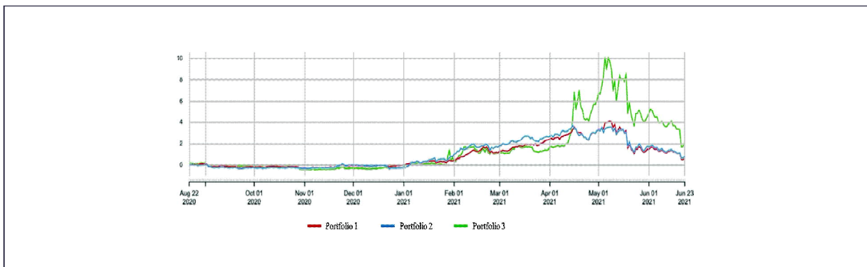
Figure 19: Cumulative Return for Portfolio 1, 2 and 3
